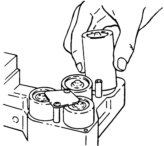
Figure 3-2. Battery Replacement
